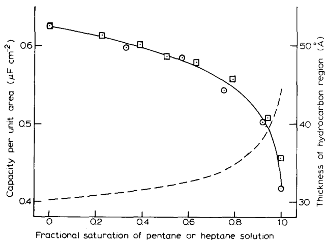
Fig. 3. The influence of n -pentane and n -heptane on the electrical capacity per unit area and hydrocarbon layer thickness of monoolein-cholesterol-hexadecane films. Capacity in n -pentane, (□) and n -heptane, (○). The dashed curve indicates the thickness variation. The film-forming and aqueous phases were equilibrated before the experiments. Bulk partition coefficients for the hydrocarbons were assumed independent of concentration. For n -pentane, the capacities are possibly erroneously high and the thicknesses low owing to the difficulty of ensuring equilibrium when using volatile solvents.
