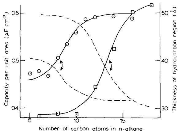
Fig. 2. The variation in electrical capacity per unit area, and hydrocarbon layer thickness of black lipid films formed with different n -alkanes. □, capacity of egg phosphatidylcholine films in absence of cholesterol (the points for decane-octadecane are taken from ref. 13); ○, capacity of egg phosphatidylcholine films containing cholesterol/phosphatidylcholine = 0.4. The dashed curves show the thickness variations and are related to the full curves as indicated by the arrows. The aqueous phase was as in Fig. 1.
